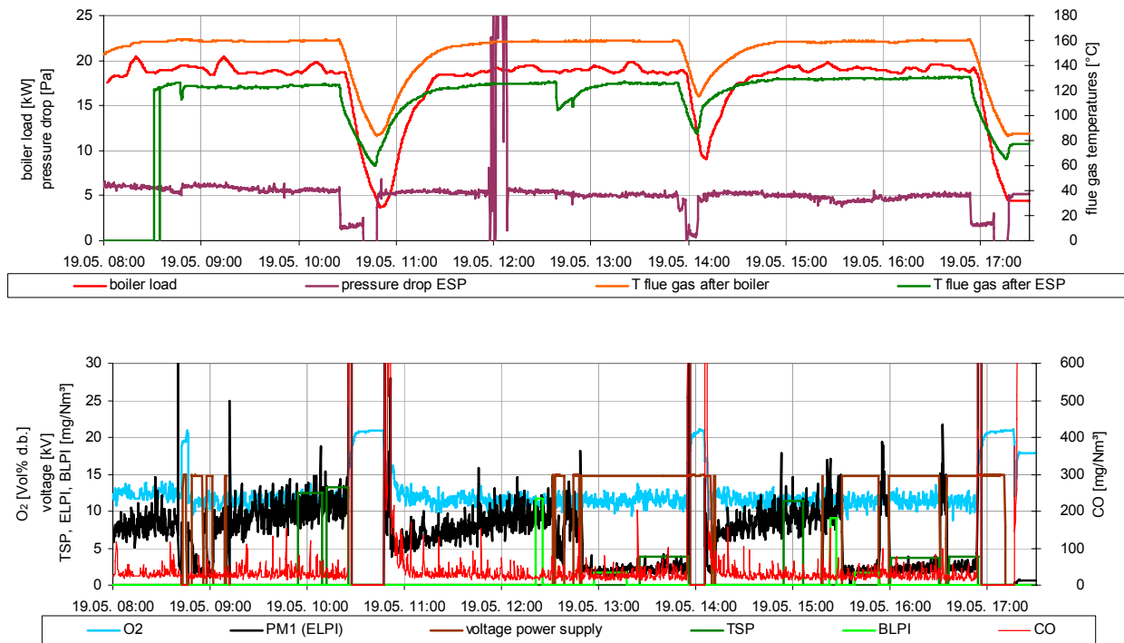
Figure 44: Results of test runs at test stand performed by BIOS and Windhager
