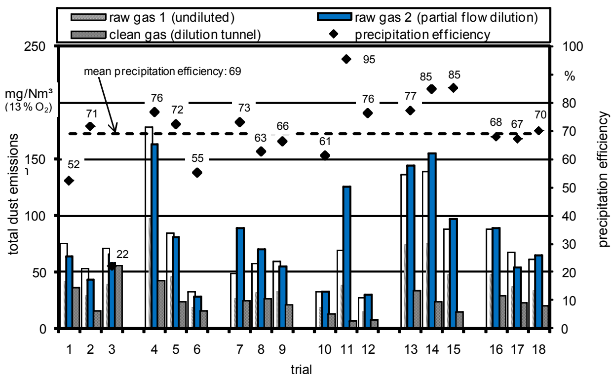
Figure 14: TSP precipitation efficiency of R_{\text{residential}} ESP – modern stove
