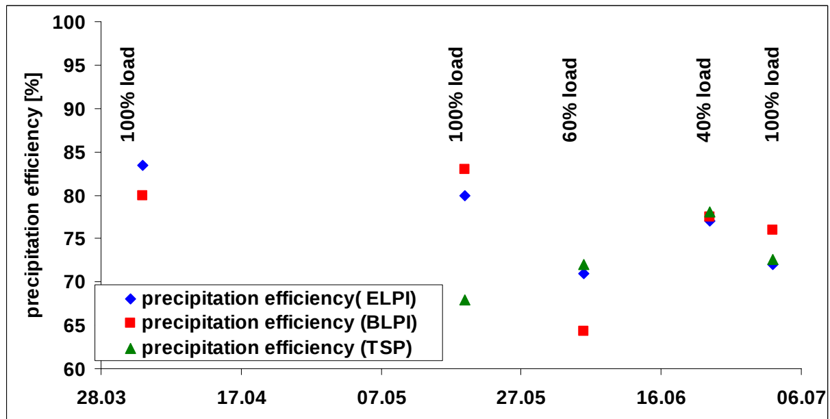
Figure 45: Precipitation efficiency of the Windhager ESP
