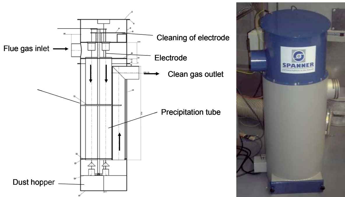
Figure 32: Scheme of the SF20 technology (left) and picture of the ESP (right)
