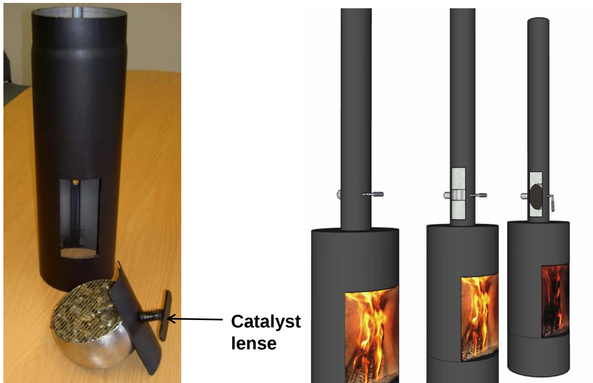
Figure 56: Picture of the catalytic converter MEKAT (left) and schemes of typical applications (right)
