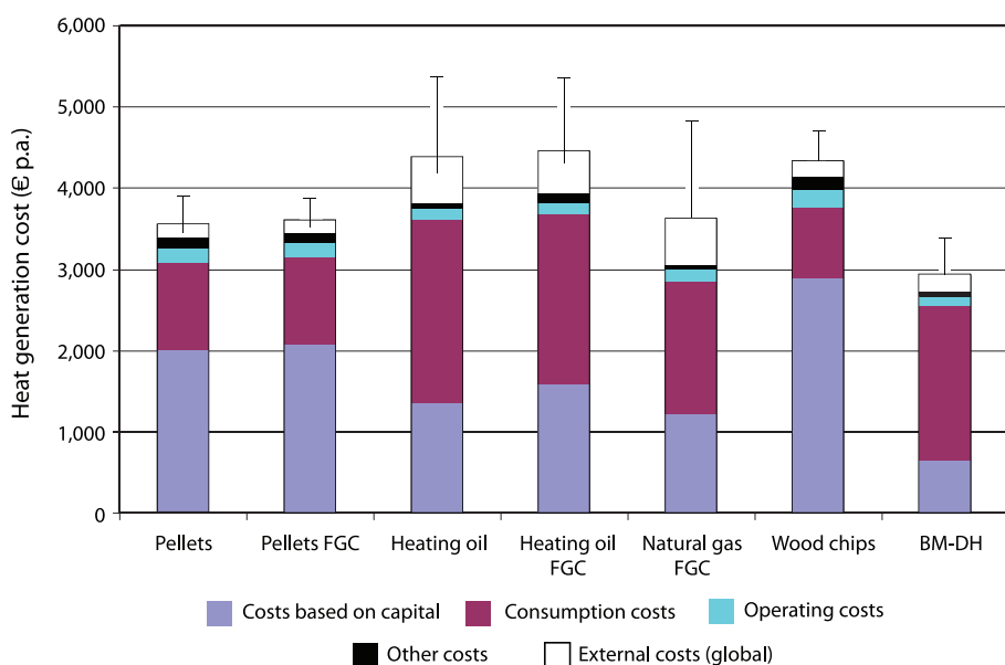
Figure 5: Specific heat generation costs of central heating systems with external costs based on global emission prognoses. [27]
