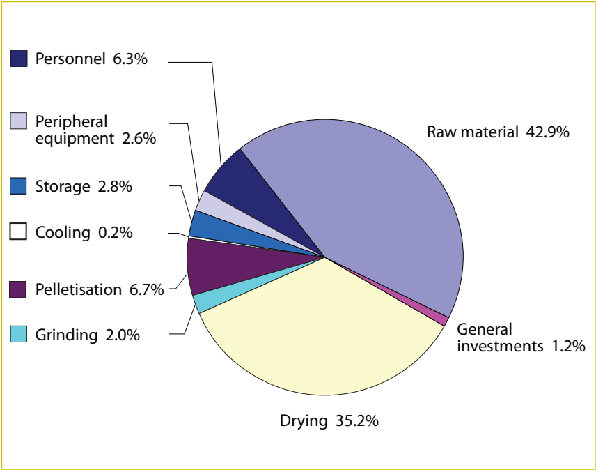
Figure 4: Pellet production costs and their composition according to the different cost factors when sawdust is used as raw material. [1]
