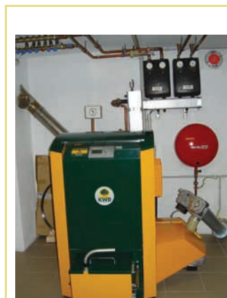
Case study 2: Pellet central heating system
